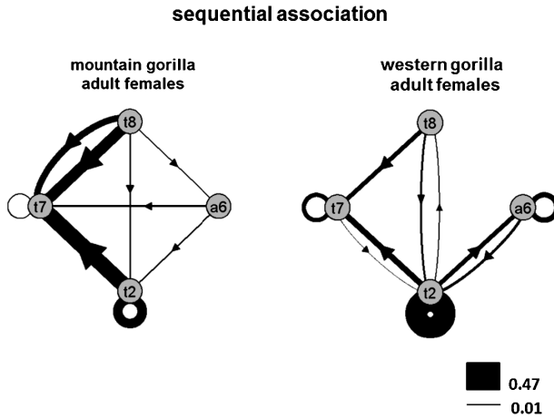
Figure A6. Sequential associations between unit types in the adult females of both gorilla groups. Lines indicate the average Dice index of sequential association as a measure of how frequently any two unit types followed one another in immediate succession. Average values were calculated from the individuals' Dice indices for a given pair of unit types. The legend depicts the thickness of the lines corresponding to the minimum and maximum average Dice index. Included are only unit types shared by all adult females.
