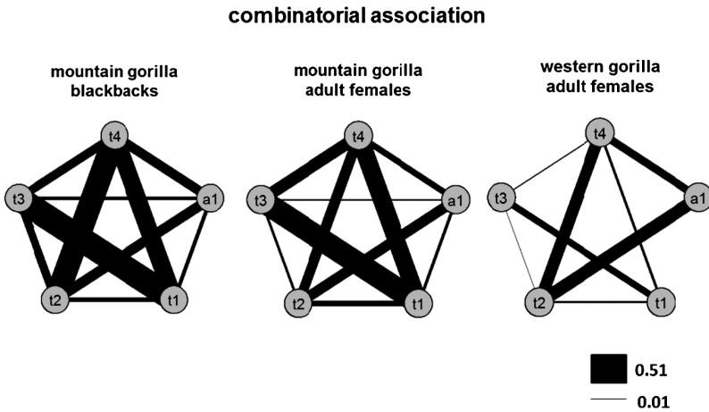
Figure 4. Combinatorial associations between unit types in both gorilla groups. Lines indicate the average Dice index of combinatorial association as a measure of how frequently any two unit types were observed together in the same call. Average values were calculated from the individuals' Dice indices for a given pair of unit types. The legend shows the thickness of the lines corresponding to the minimum and maximum average Dice index.
