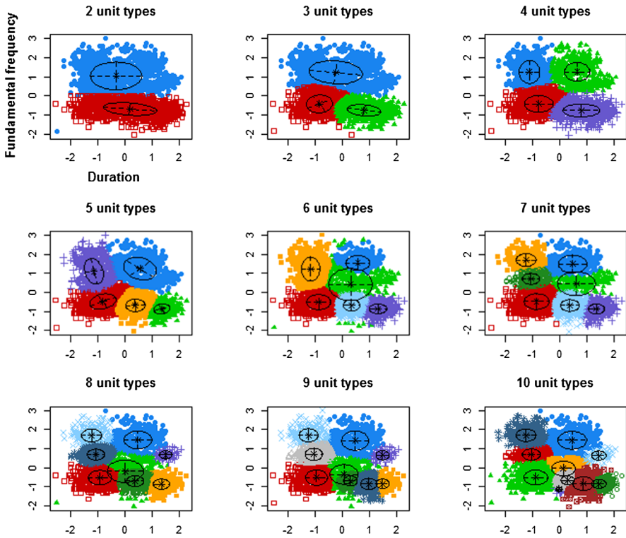
Figure A5. Best cluster solutions for 2 to 10 unit types (clusters) of tonal units. Indicated are the values of the principal component for acoustic parameters describing the fundamental frequency on the y-axis and the transformed duration on the x-axis. Different colours and symbols indicate different clusters. For each cluster the cluster mean is marked and ellipses indicate corresponding covariance. Note that an increase in the number of clusters usually largely lead to a split of a certain cluster rather than a more fundamental change in the arrangement of units into clusters.
