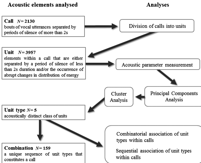
Figure 2. Operational definitions and schematic overview of analyses used in this study.
