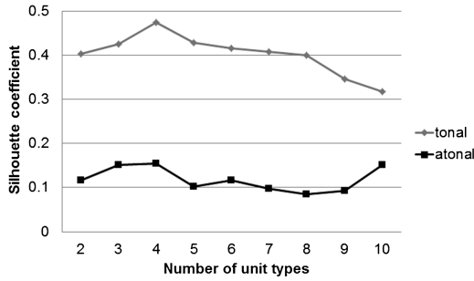
Figure A3. Silhouette coefficients of the different cluster solutions for tonal and atonal units as a function of the number of unit types (clusters). A silhouette coefficient < 0.25 indicates strong intergradation, silhouette coefficients between 0.25 to 0.5 weak clustering.
