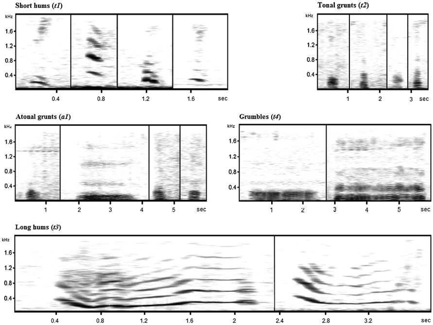
Figure 3. Spectrograms of the 5 unit types. Short hums (t1) were usually under 1-s short, tonal, high pitched units. Tonal grunts (t2) were short, low pitched grunts. Atonal grunts (a1) were on average short, noisy grunts that, however, could be up to 2 s long. Grumbles (t4) were up to 5 s long and low pitched. Long hums (t3) were long tonal, high pitched units.
