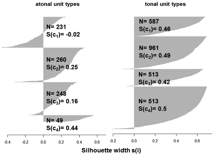
Figure A4. Silhouette plots illustrating the most discrete cluster solutions with four unit types (clusters) for atonal units, with an overall silhouette coefficient of 0.15 (left) and with four unit types for tonal units, with an overall silhouette coefficient of 0.48 (right). The plot displays the silhouette widths for each unit as horizontal bars, ordered by clusters and by silhouette value within cluster. The silhouette width is a measure of how clearly a unit belongs to its assigned cluster. Compact clusters consist of units with high silhouette widths. N indicates the number of units allocated to each cluster. S ( c n ) is the silhouette coefficient of each cluster.
