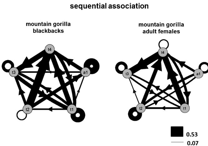
Figure 5. Sequential associations between unit types in the blackbacks and adult females of the mountain gorilla group. Lines indicate the average Dice index for sequential association as a measure of how frequently any two unit types followed one another in immediate succession. Average values were calculated from the individuals' Dice indices for a given pair of unit types. The legend depicts the thickness of the lines corresponding to the minimum and maximum average Dice index. For reasons of clarity illustrations include only transitions with a Dice index > 0.05.
