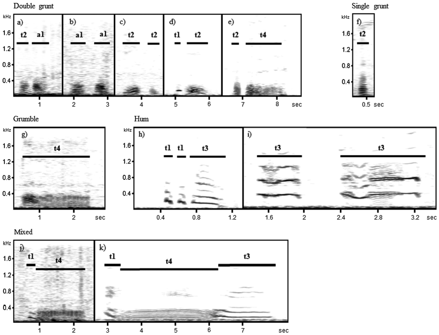
Figure 1. Spectrograms of representative gorilla close calls recorded in this study, their subdivision into units and categorization into unit types. Spectrograms a–f illustrate typical examples of syllabled calls: (a–e) double grunts, (f) single grunt. Spectrograms g–k illustrate non-syllabled calls: (g) grumble; (h, i) hums; (j, k) mixed calls. Calls were subdivided into units (indicated by black lines) based on the occurrence of periods of silence of less than 2 s duration (a–e, h, i) or abrupt changes in the distribution of energy (j, k). The units were categorized as atonal or tonal according to the presence/absence of harmonic frequency bands. Indicated above the lines are the unit type each unit was assigned to via cluster analysis: a1, atonal grunts; t1, short hums; t2, short tonal grunts; t3, long hums; t4, grumbles.
