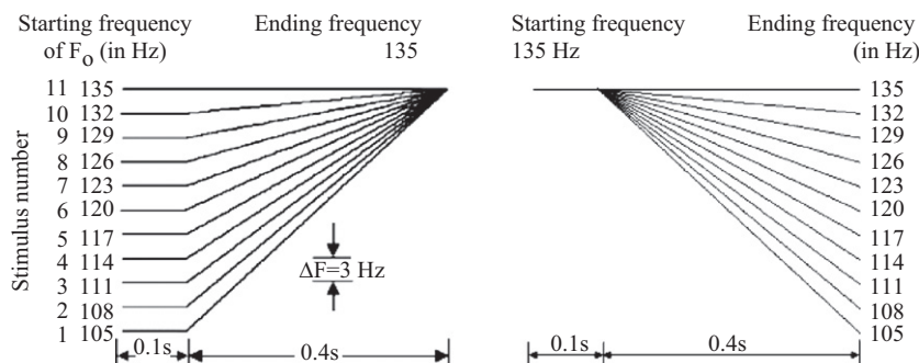
Fig. 1. Tone contours for the stimuli in the two types of continuum: left for the rising continuum, and right for the falling continuum.
