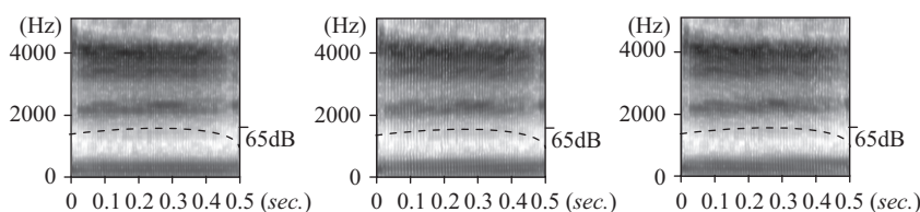
Fig. 2. Resynthesized speech (Mandarin /i/ syllables). The panels show the wideband spectrogram of the Number 11 speech stimulus (left), the Number 1 stimulus of the rising speech continuum (middle), and the Number 1 stimulus of the falling speech stimuli (right). The thin dashed lines indicate the intensity profiles.
