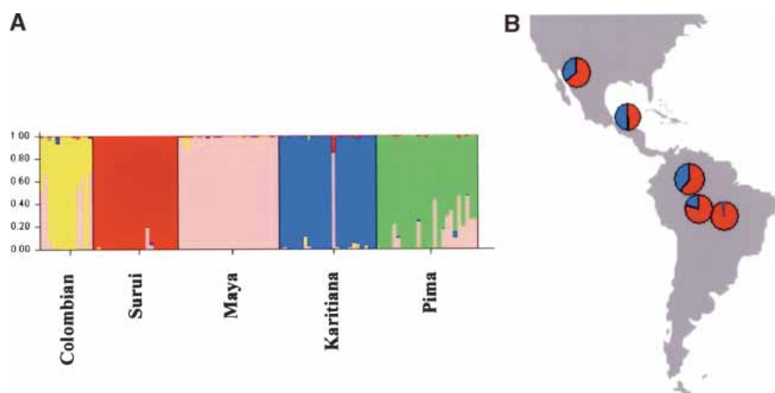
Figure 4 Assignment of Native American individuals using (A) correlated allele frequencies as used in Rosenberg et al. (2002) and (B) uncorrelated allele frequencies. In B, the assignment of the individuals has been determined using all individuals from the first subsample and four inferred populations as in Figure 2. In A, each bar represents a single individual, and the colors correspond to the coefficients of ancestry. In B, the coefficients of ancestry were averaged over the five individuals for each population. Blue and red segments represent the proportion of ancestry in inferred population B and D, respectively.
