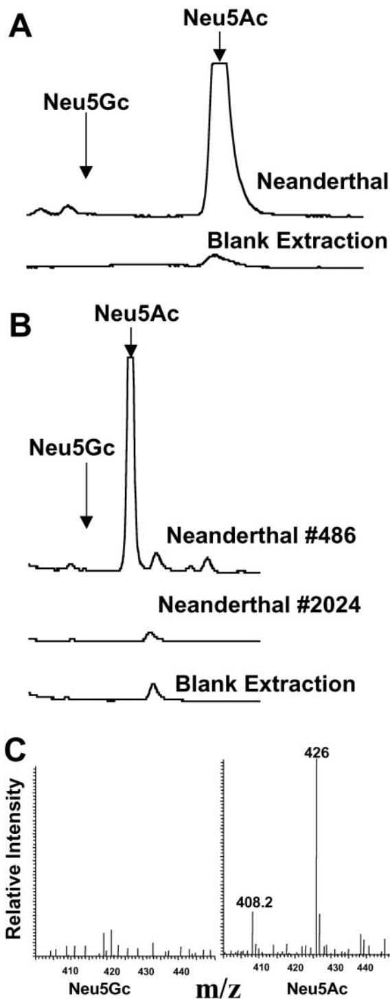
Fig. 3. Sias from Neandertal fossils. Sias were released, purified, and characterized as in Fig. 2. (A) HPLC profile of extract from the original Neandertal-type specimen. The wash through blank is a control for human handling. The column was deliberately overloaded to take the Neu5Ac peak off scale, highlighting the absence of Neu5Gc. (B) HPLC profile of Sias from Georgian Neandertals. The absence of Sias from sample ID no. 2024 was confirmed by MS analysis. (C) MS of Neu5Ac peak from sample ID no. 486 showing m/z corresponding to the hydrated (426) and dehydrated (408) DMB derivatives of Neu5Ac. There were no detectable ions corresponding to Neu5Gc derivatives (442 or 424).
