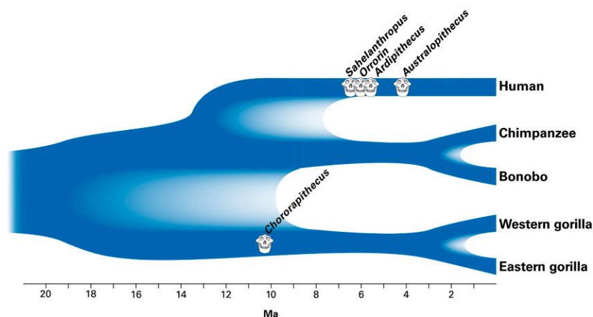
Fig. 1. Diagram illustrating the branching pattern and timing of the splits between humans, chimpanzees, bonobos, western gorillas, and eastern gorillas. The paler shading indicates the range of split times inferred in this study. Cartoon skulls indicate approximate age of the indicated fossil remains, but do not imply that these fossils were necessarily on those ancestral lineages or that entire crania actually exist for these forms.
