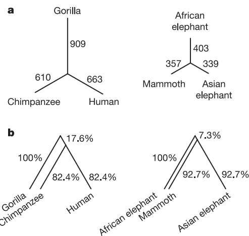
Figure 3 | Comparison of three-species trees. Comparisons based on the complete mtDNA sequences for human, chimpanzee, gorilla, mammoth and African and Asian elephants. a, Absolute number of phylogenetically informative positions on which the three-species test is based. b, Relative length of the internal branch in the two groups of species for clock-like phylogenetic trees using the substitution data from a and rooted by midpoint rooting. Note the differences in the absolute numbers of substitutions and relative branch length of the internal branch between the two species groups (see also Supplementary Information).
